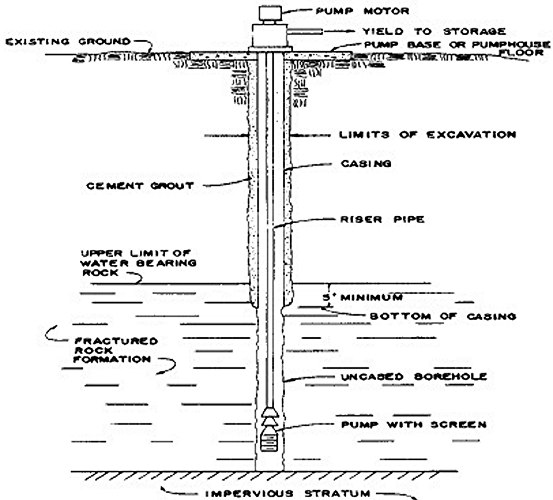
Figure 5-6 Well in Rock Formation
