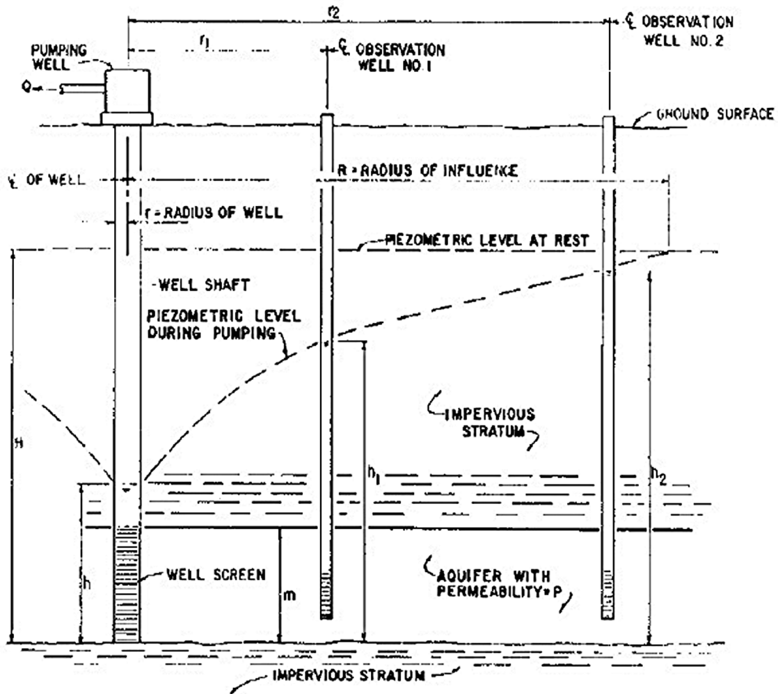
Figure 5-3 Diagram of Water Table Well (unconfined aquifer)
