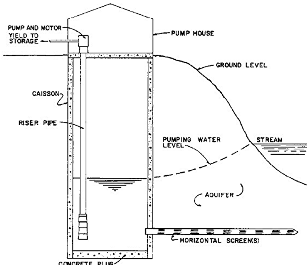
Figure 5-2 Collector Well
